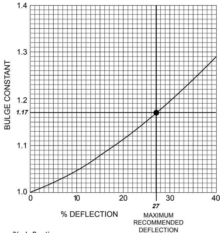
BULGE CURVE
